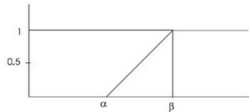
Figure 2: An example of the function \Gamma
